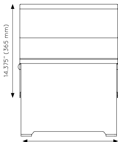
front view of the step in the raised position
