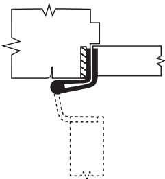
SWING CLEAR Full Mortise; Wood Door/ Hollow Metal Jamb
