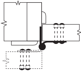
HALF SURFACE Wood Door/ Wood Jamb
