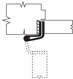
SWING CLEAR Half Surface; Mineral Core Door/ Hollow Metal Jamb
