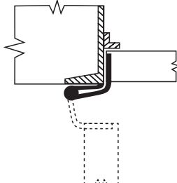
SWING CLEAR Half Mortise; Wood Door/ Channel Iron Jamb
