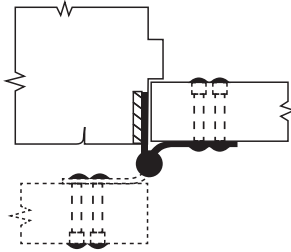
HALF SURFACE Mineral Core Door/ Hollow Metal Jamb
