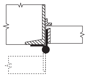
HALF MORTISE Hollow Metal Door/ Channel Iron Jamb
