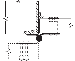
FULL SURFACE Hollow Metal Door/ Channel Iron Jamb
