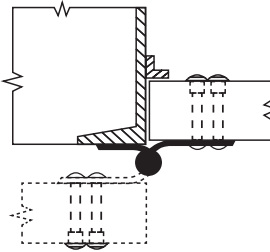
FULL SURFACE Mineral Core Door/ Channel Iron Jamb
