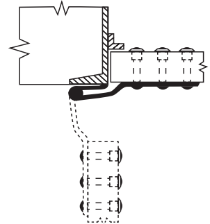
SWING CLEAR Full Surface; Mineral Core Door/ Channel Iron Jamb
