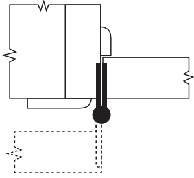
FULL MORTISE Wood Door/ Wood Jamb
