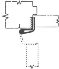
Swing Clear Half Surface; Mineral Core Door/Hollow Metal Jamb
