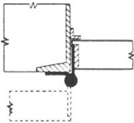
Half Mortise; Hollow Metal Door/ Channel Iron Jamb
