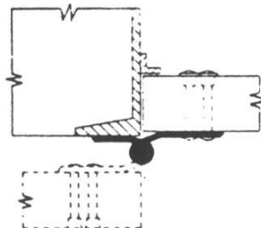
Full Surface; Hollow Metal Door/Channel Iron Jamb
