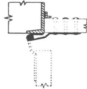
Swing Clear Full Surface; Mineral Core Door/ Channel Iron Jamb
