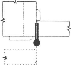
Full Mortise; Wood Door/Wood Jamb
