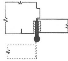
Full Mortise; Hollow Metal Door/Hollow Metal Jamb
