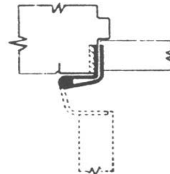
Swing Clear Full Mortise; Wood Door/Hollow Metal Jamb
